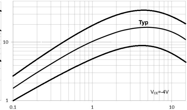
h_{FE}-I_C BL15P15A (Typical)
